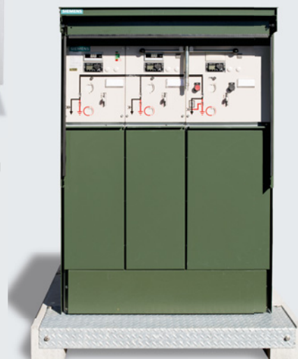
Siemens 8DJH Outdoor Class A on concrete flat pad
