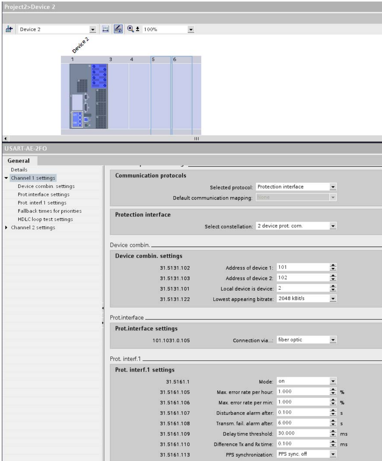
Figure 4: Settings for the PI-interface on module location F for device 2.
